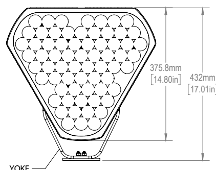
*SM200 bracket mounting option shown. See page 2 for more mounting options.
