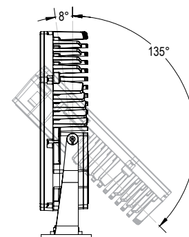
*SM200 bracket mounting option shown. See page 2 for more mounting options.
